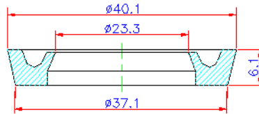
Gaxeta ref. 2003306084014 DLDB 5148413
