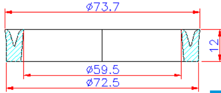
Gaxeta ref. 2003306084014 DLDB 5148413
